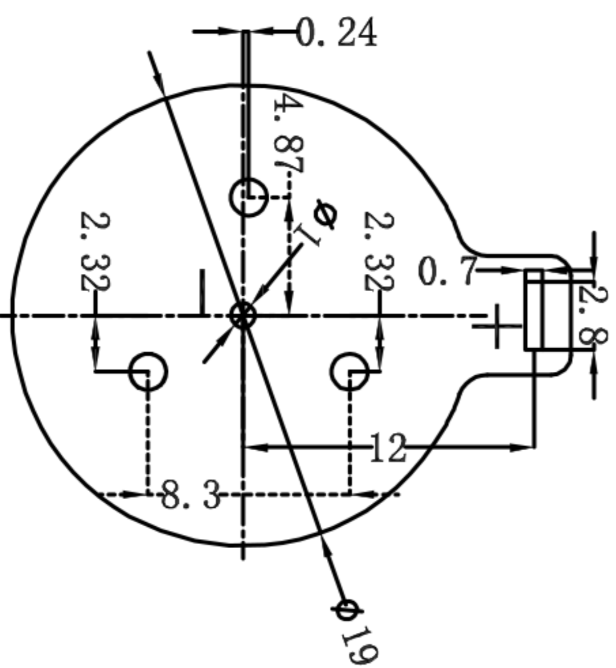
PCB Layout Diagram Top View
