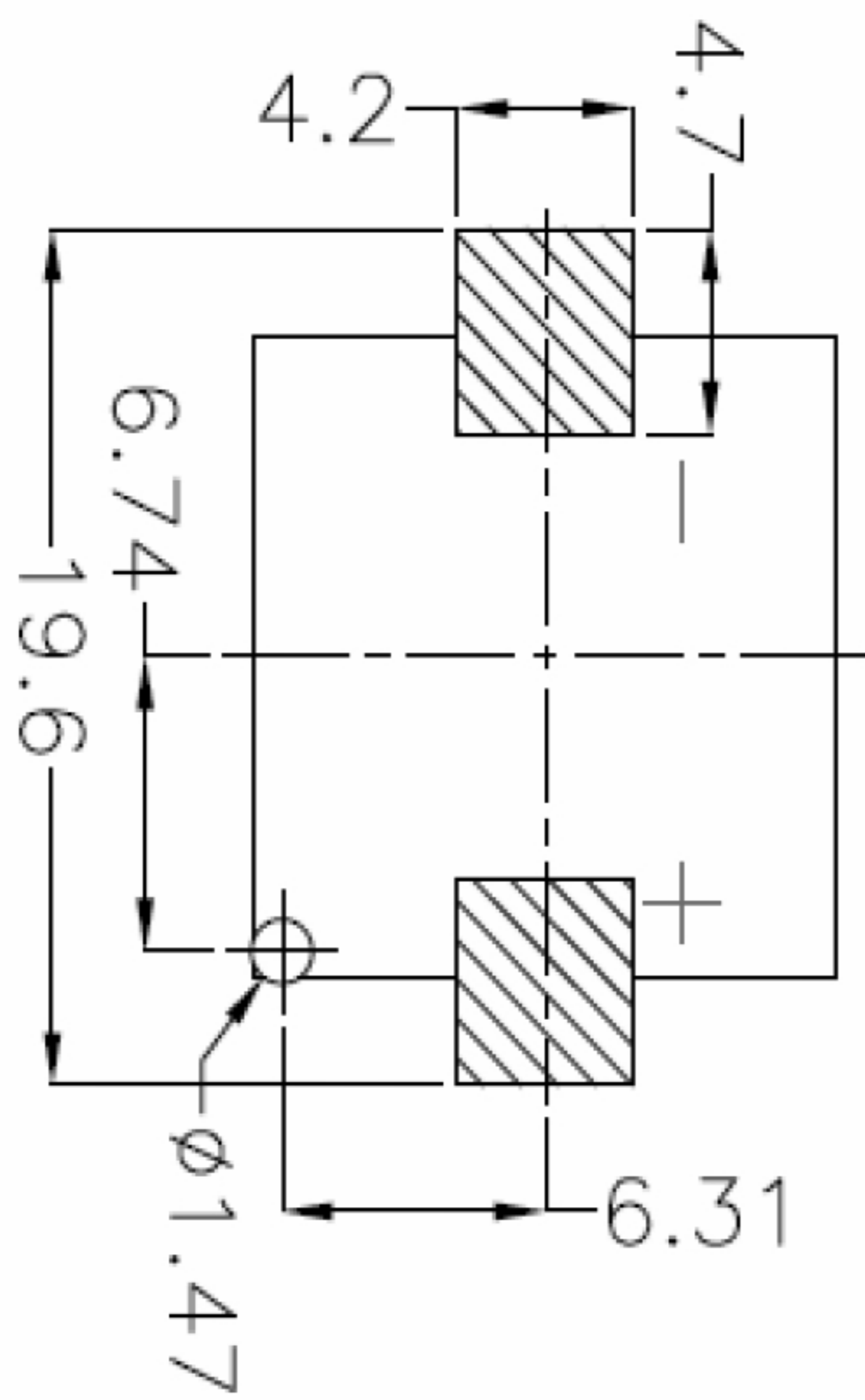
PCB Layout Diagram Top View
