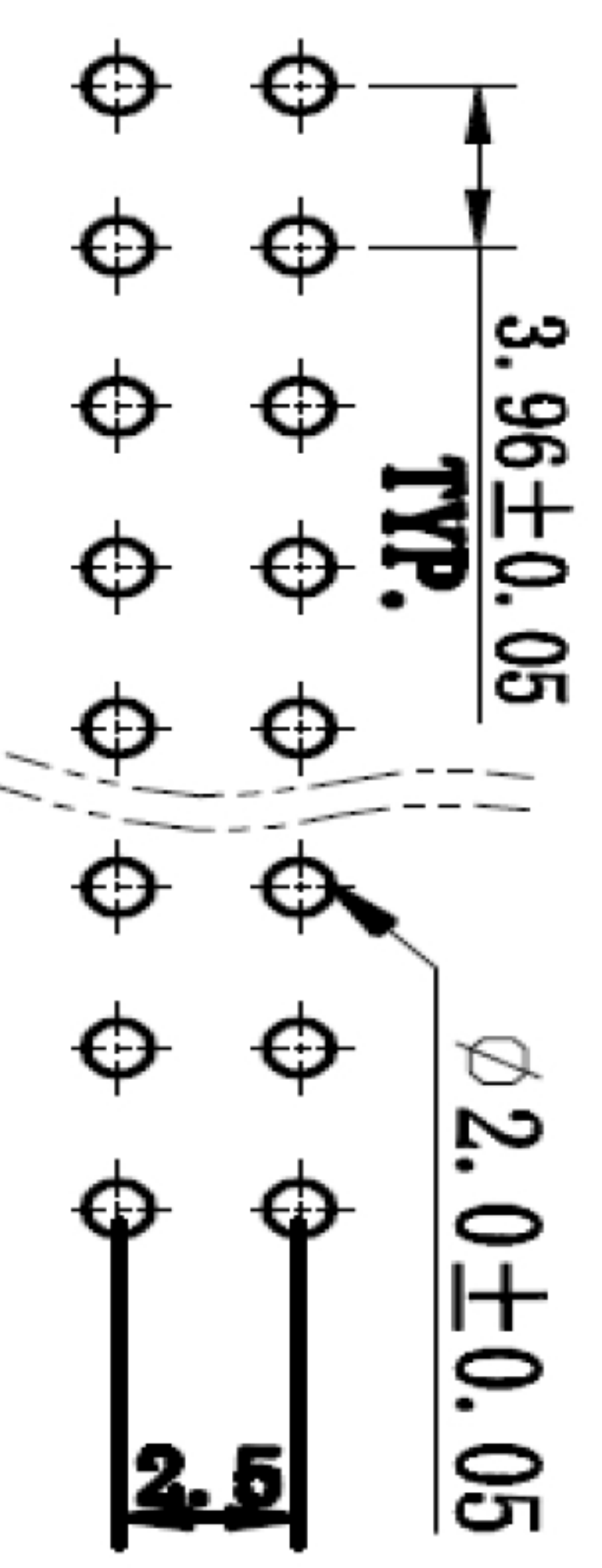
PCB LAYOUT
