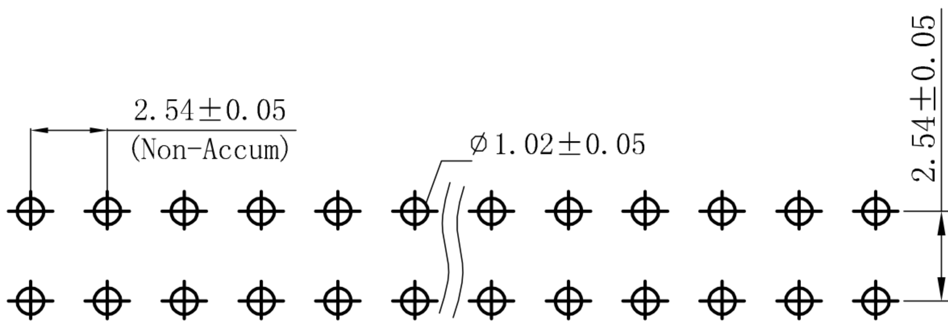
PCB LAYOUT
