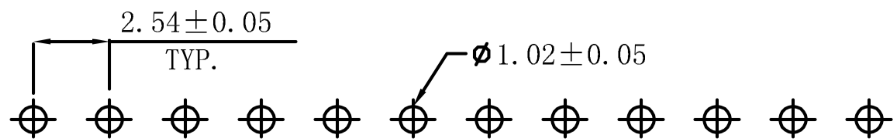
PCB LAYOUT
