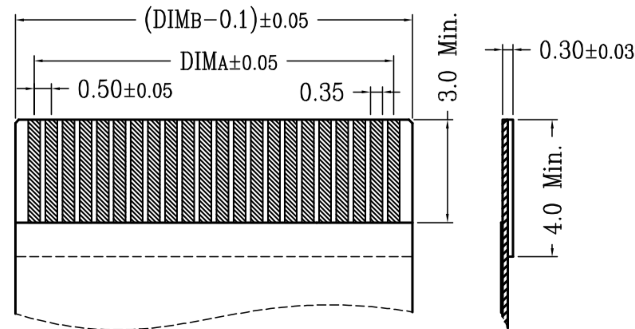
适用扁平线 (Applicable Flat Cable)
