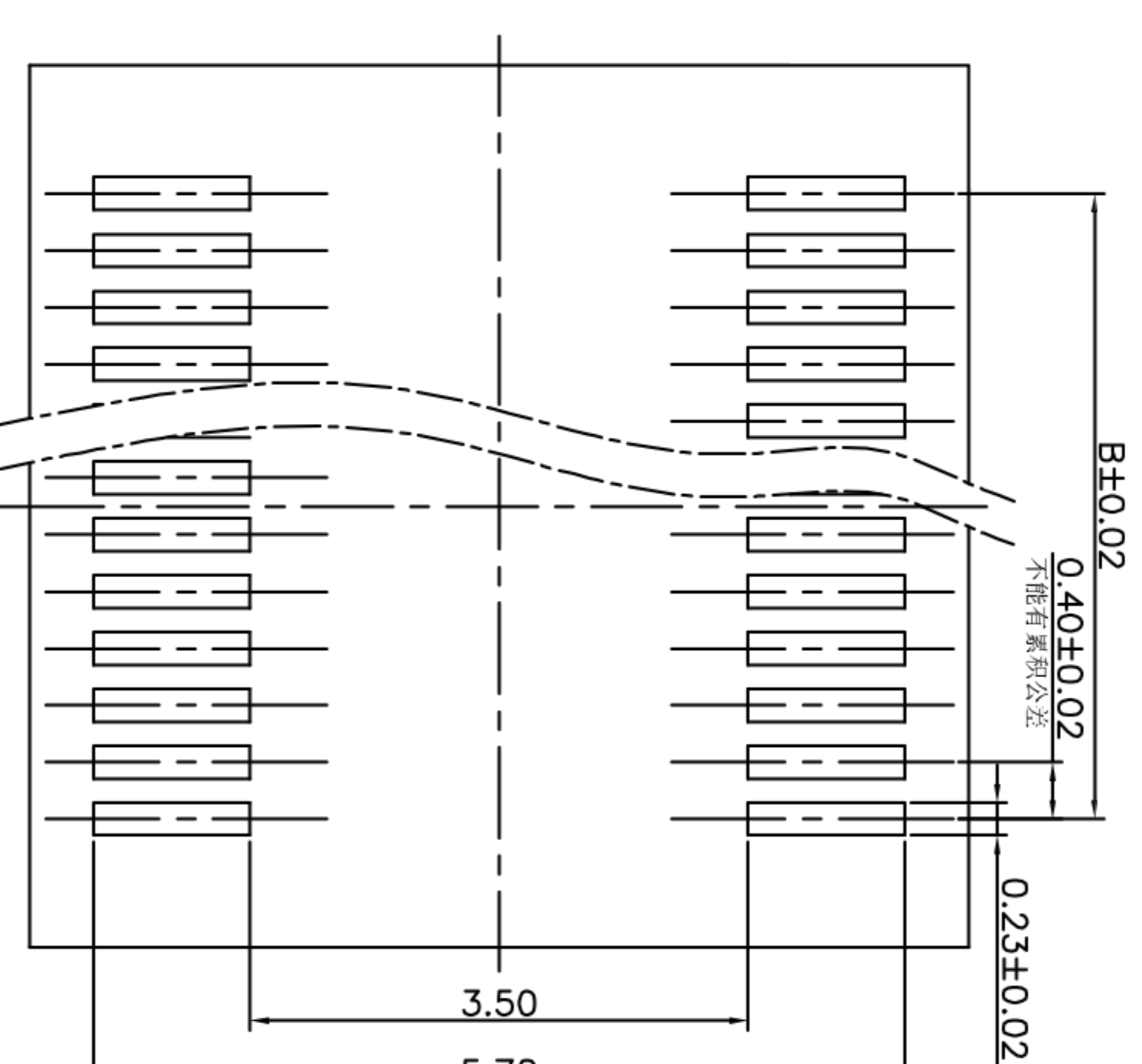
RECOMMENDED PCB LAYOUT TOP VIEW (TOLERANCE:±0.05)
